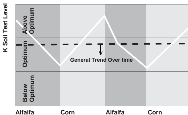
Figure 2. Soil test trends in a corn-forage rotation.
